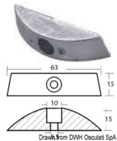
50.309 VOLVO PENTA 852018
